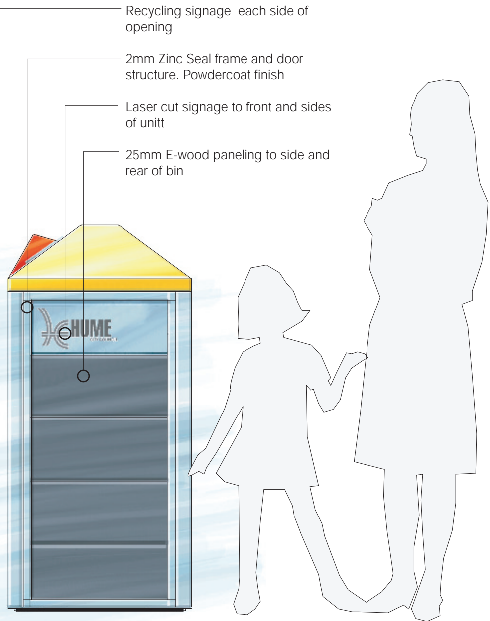
Proposed PPR unit -E-wood version Elevation NTS 28/03/08
