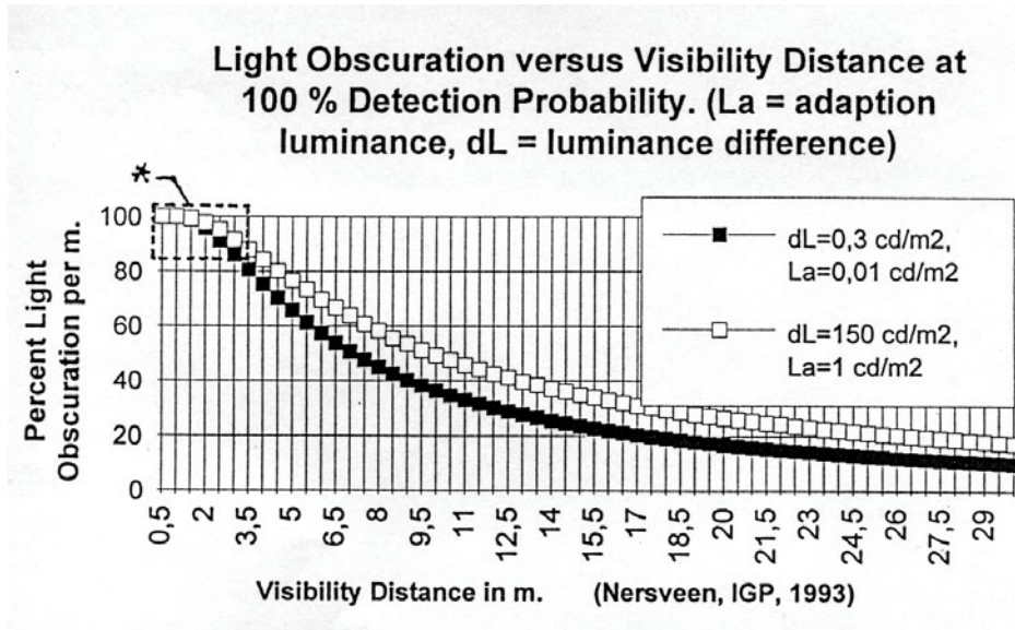
Figure 2 Visibility in heavy smoke
