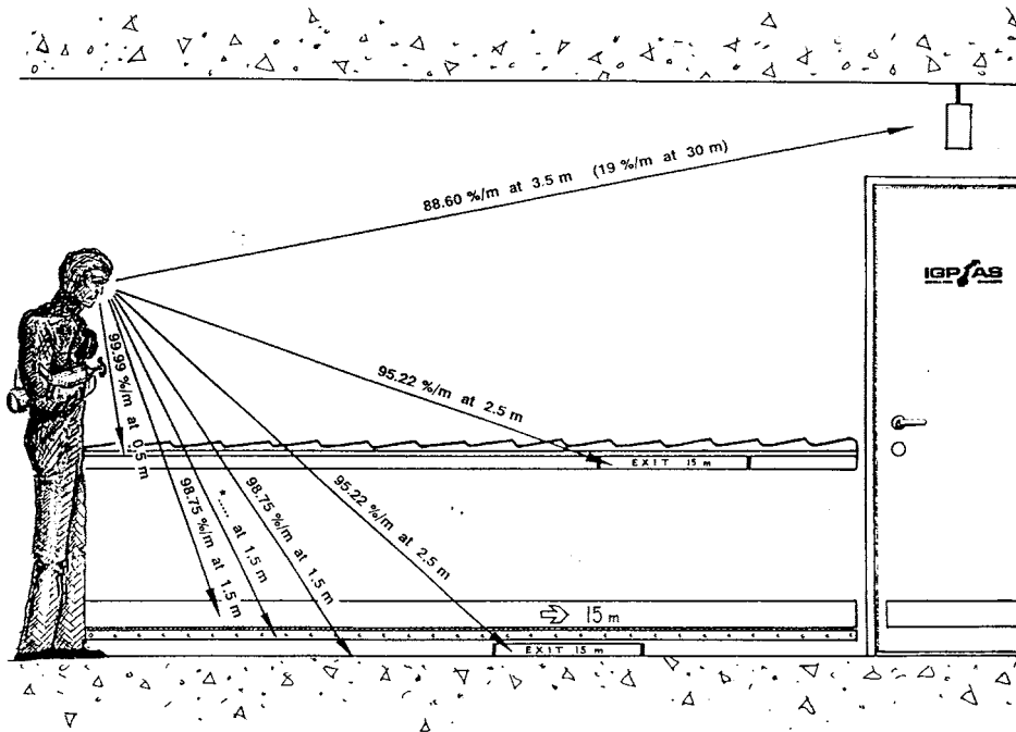
Figure 3 Smoke density and visibility in the tests
